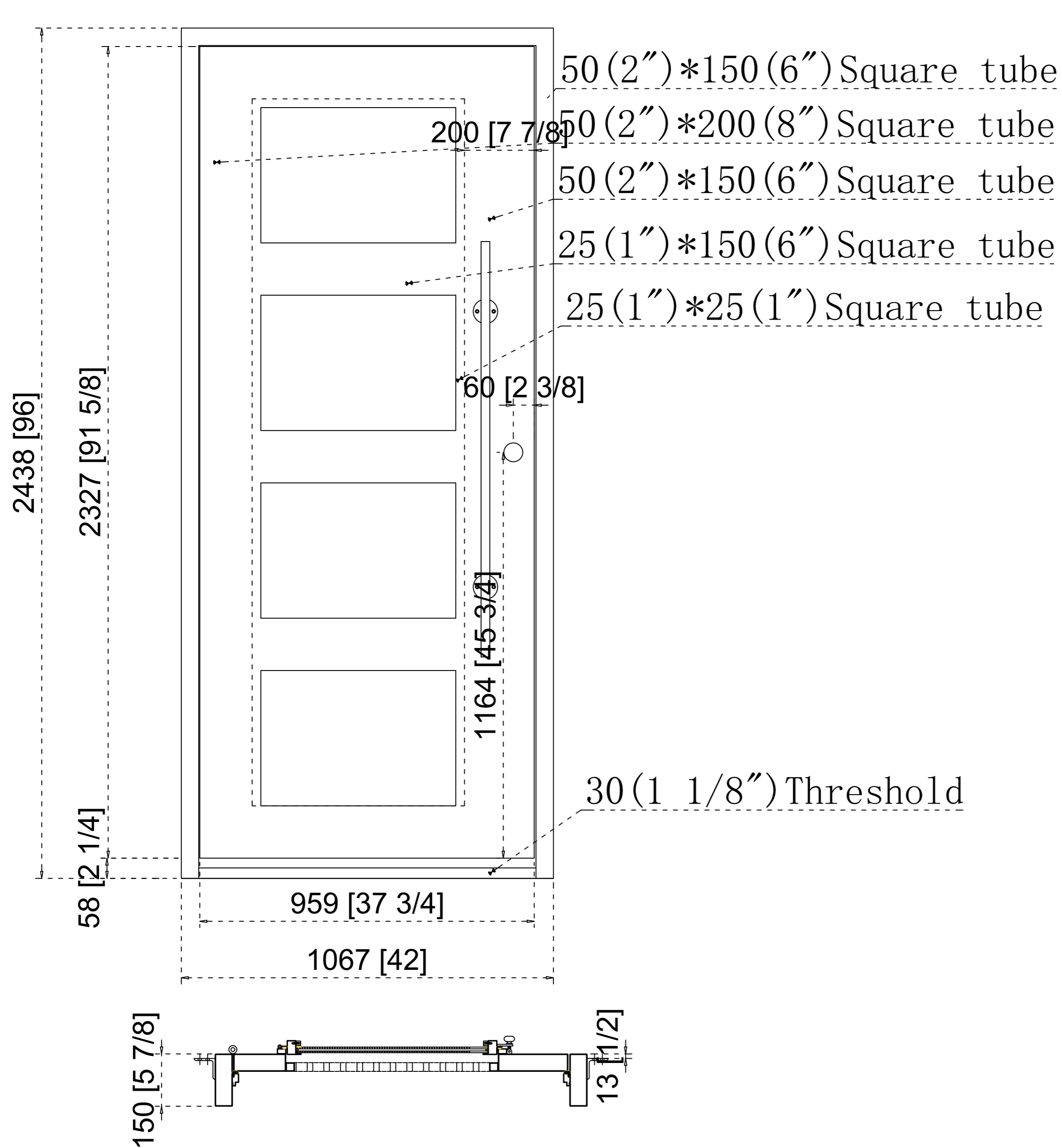
EXTERIOR VIEW
