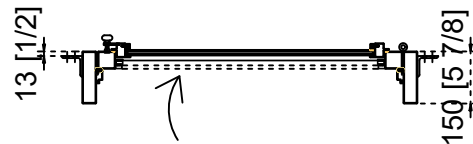
EXTERIOR VIEW
