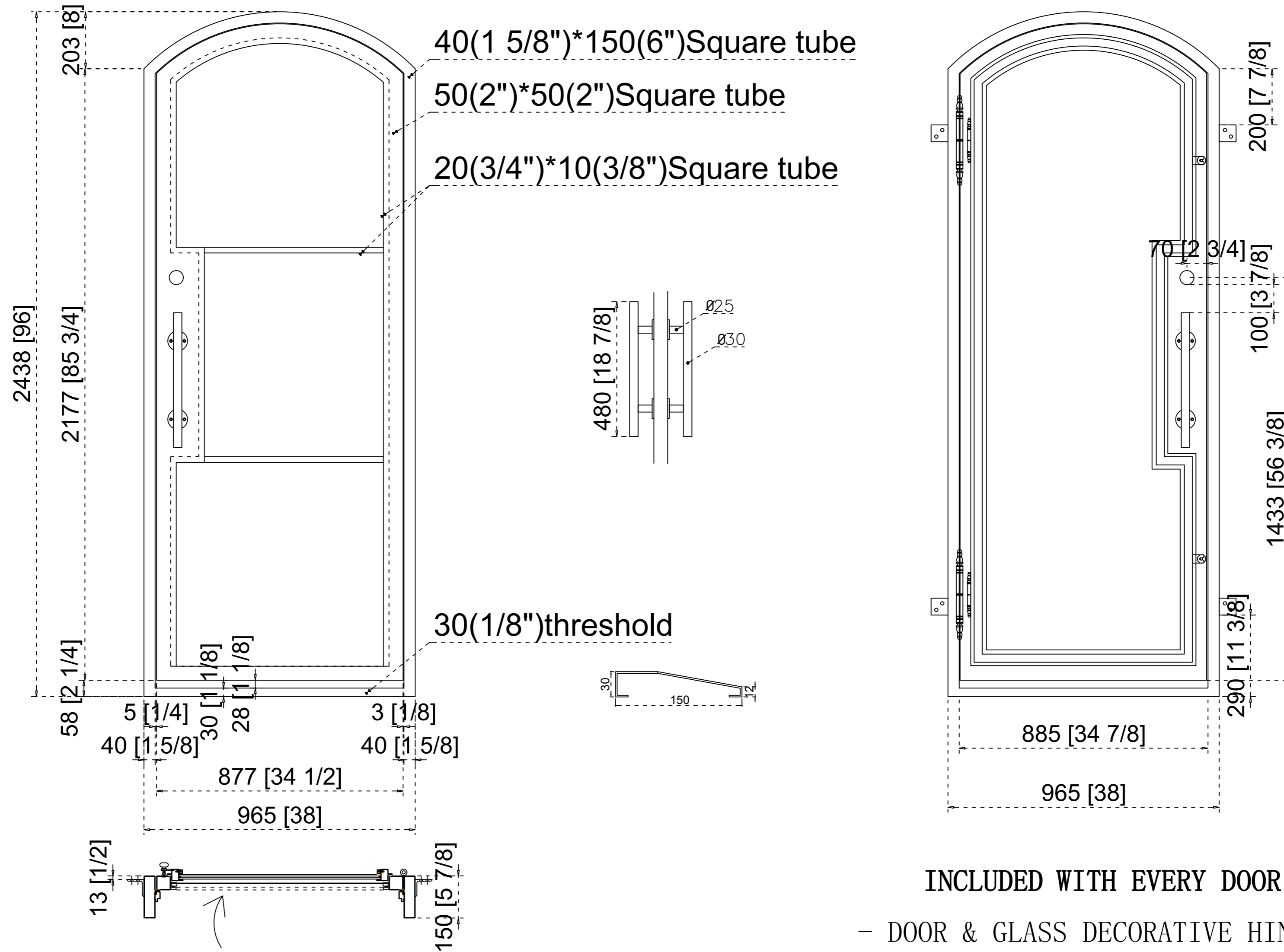
EXTERIOR VIEW
